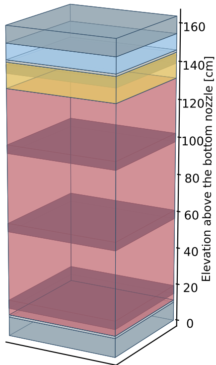
(a) Fuel assembly
