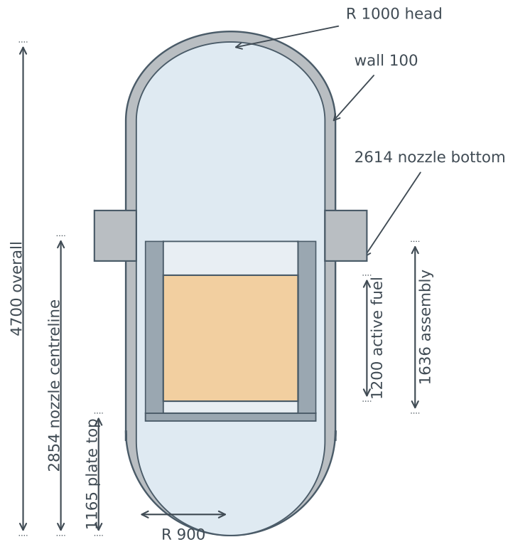
(a) Elevation, mm
