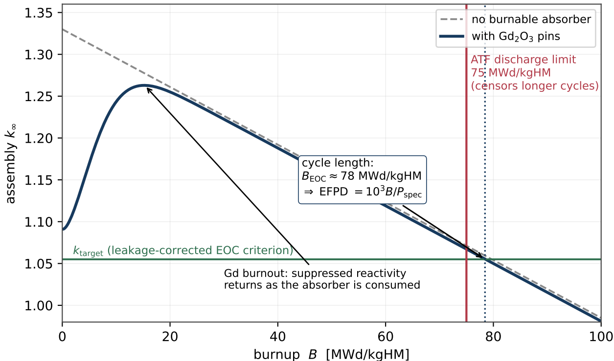
Reactivity over life: absorber hold-down, EOC target, and the burnup cap (illustrative curves)
