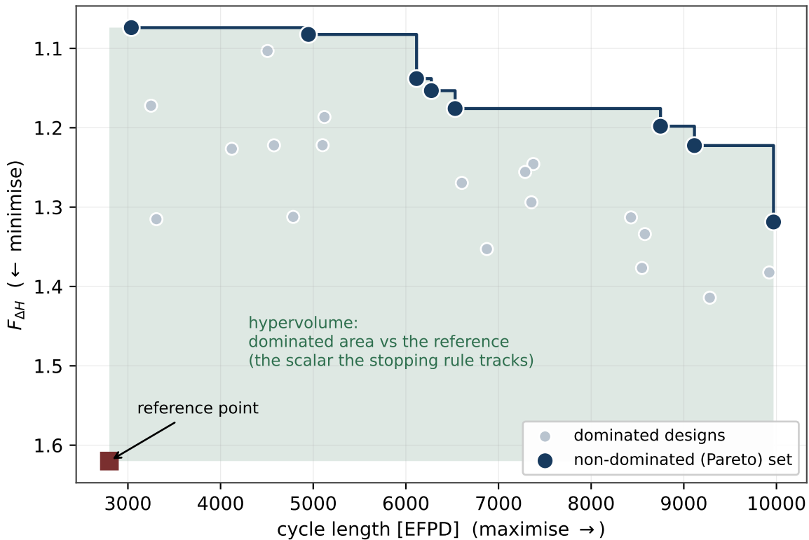
Dominance, the Pareto front, and hypervolume (synthetic data)
