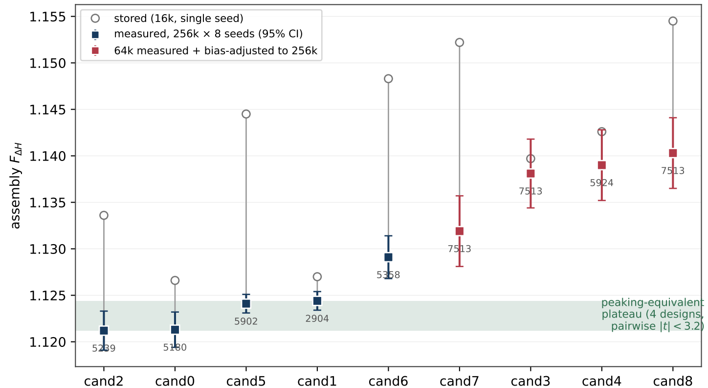
Campaign 3, high-fidelity resolution: design-dependent bias shifts (-0.003 to -0.020) re-order the set; EFPD labels under each point
