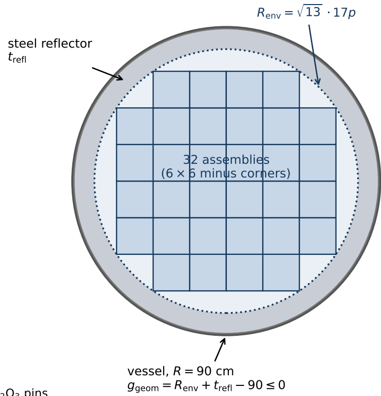
(b) core plan view (drawn at p = 1.26 cm, t_{refl} = 12 cm)
