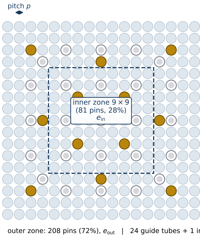
(a) 17 × 17 assembly (design variables: e_{in} , e_{out} , gd , p )
