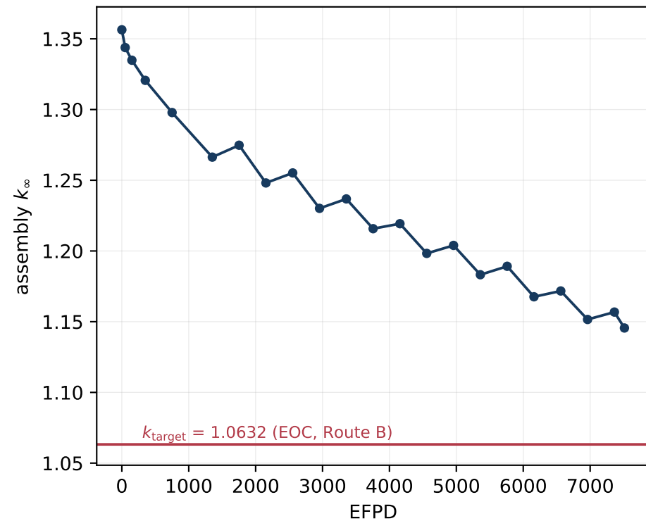
(a) idx44: measured k_{\infty} vs burnup
