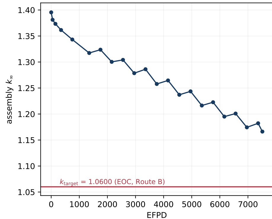
(a) idx6: measured k_{\infty} vs burnup
