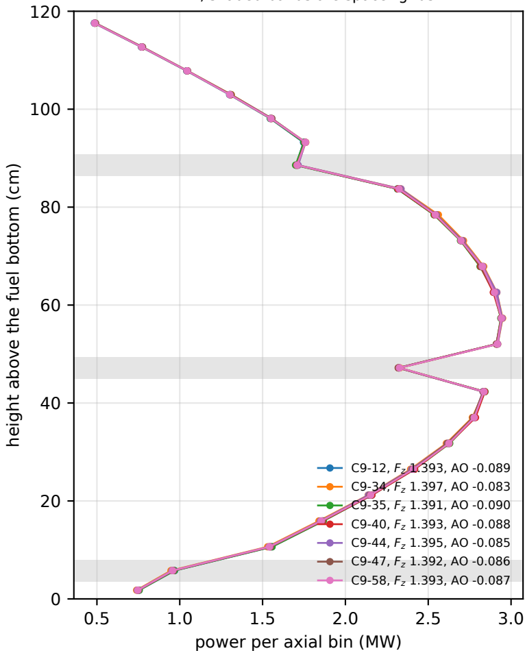
RE12, shaded bands are spacer grids
