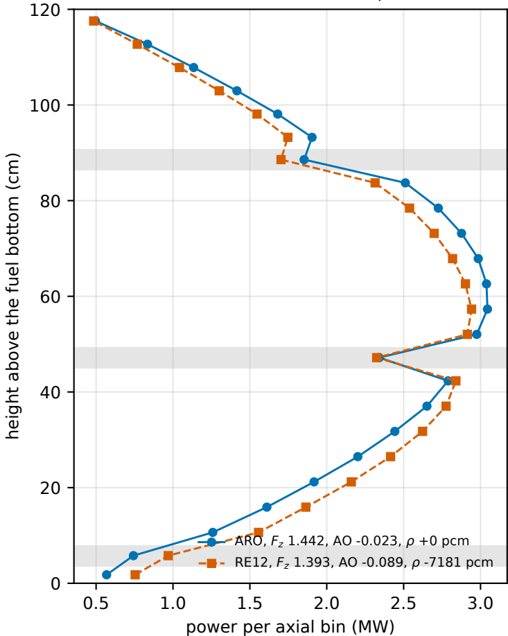
C9-12, rod effect on the axial profile
