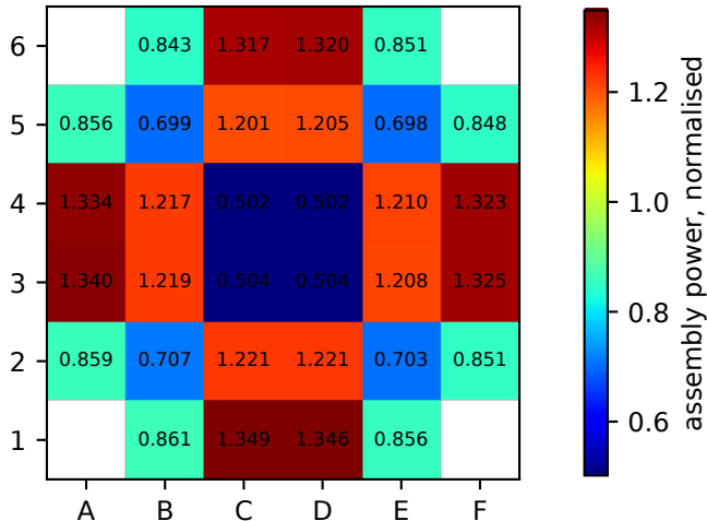
RE12, k = 0.92908
