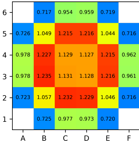
ARO, k = 0.99698
