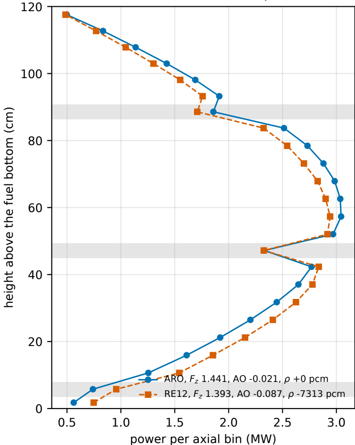
C9-58, rod effect on the axial profile
