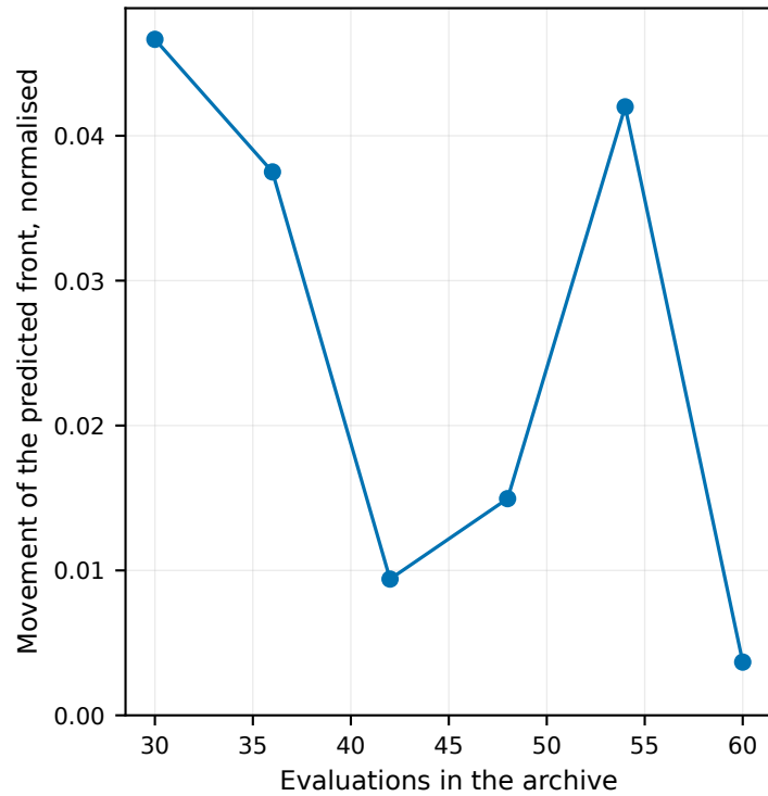
Convergence of the surrogate belief
