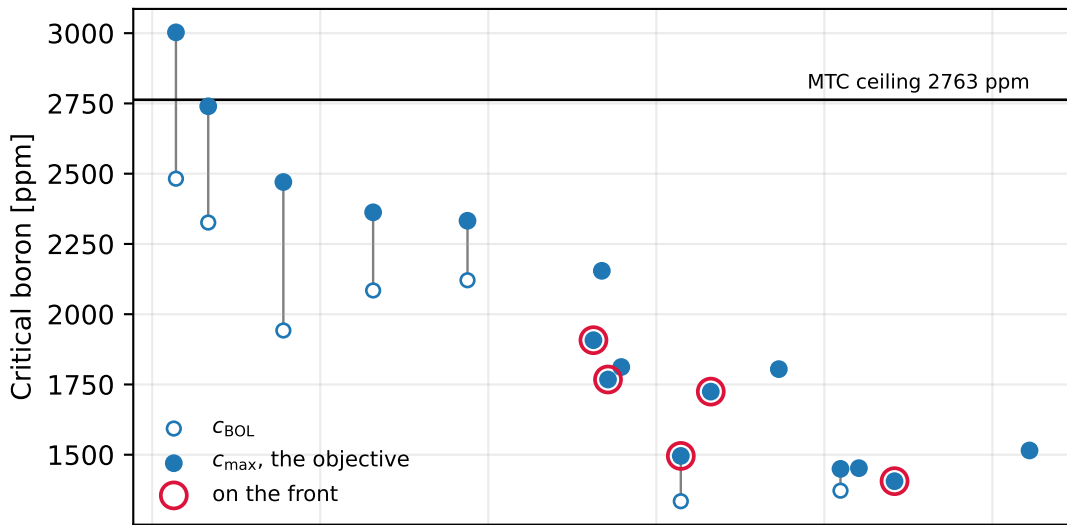
Feasible designs at 3.96 to 4.66 wt% (16 designs)
