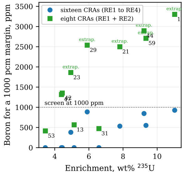
(a) boron needed at BOL
