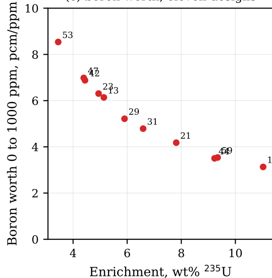
(c) boron worth, eleven designs
