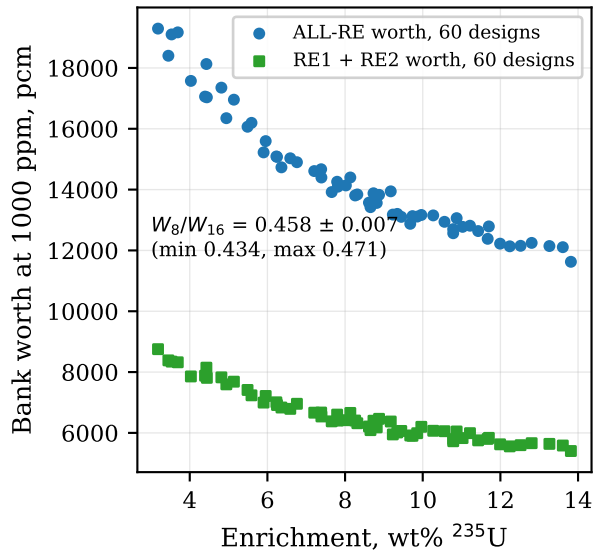
(b) regulating-bank worth
