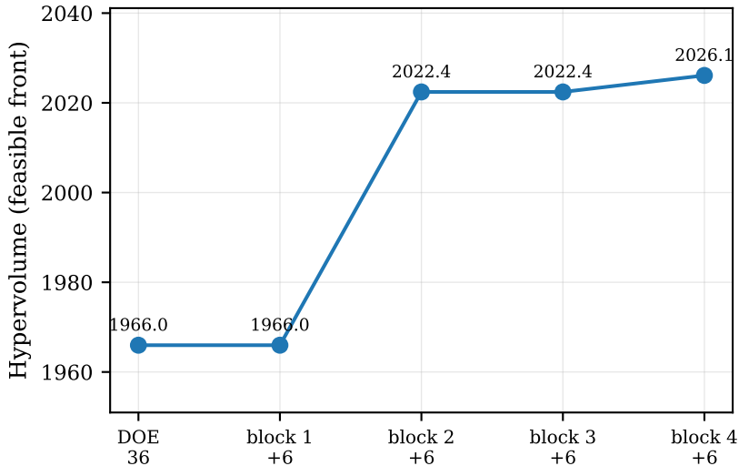
Campaign 8: reference point (EFPD 1760, F_{\Delta H} 2.096)
