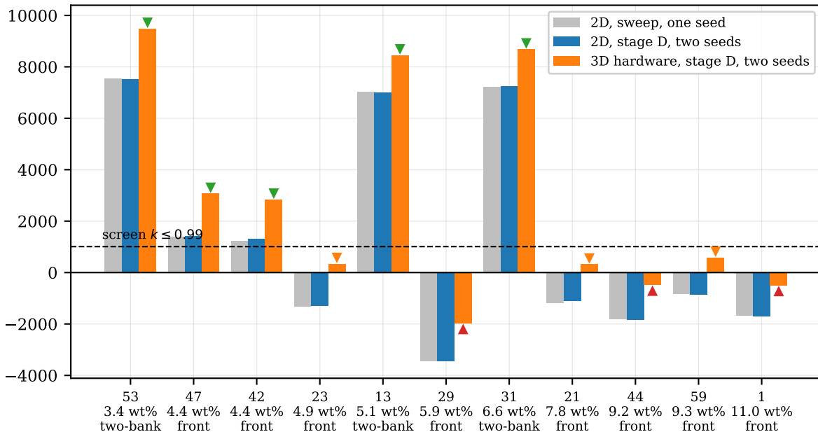
Zero-boron hold-down by the four regulating banks alone (stage D)
