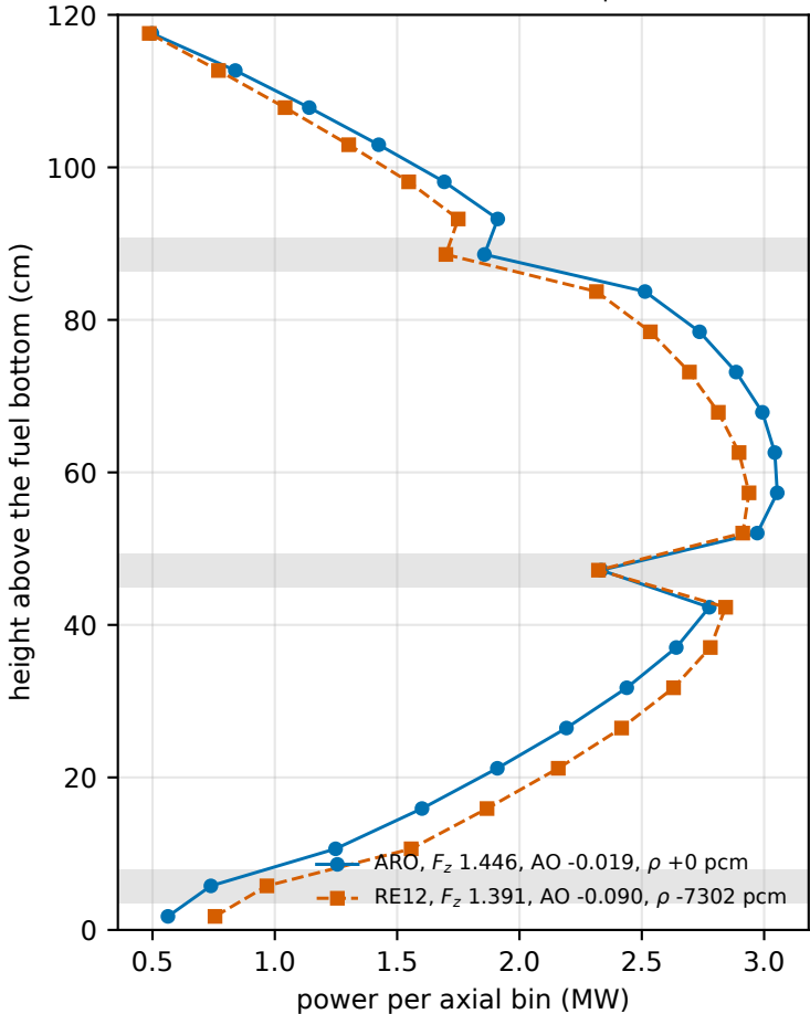
C9-35, rod effect on the axial profile
