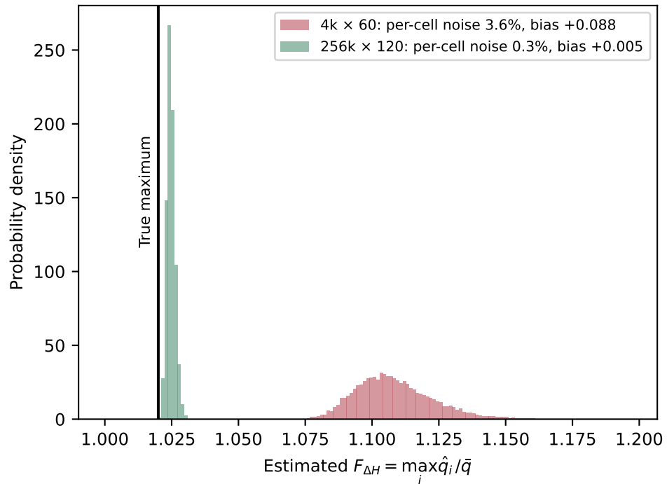
(b) Maximum over 264 noisy cells, synthetic
