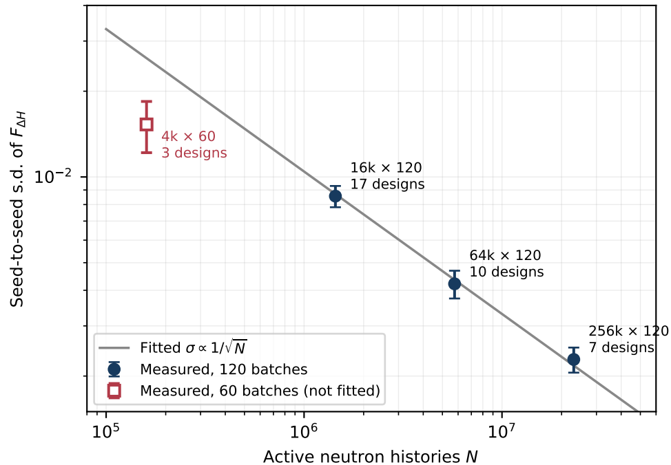
(a) Statistical error against 1/\sqrt{N}
