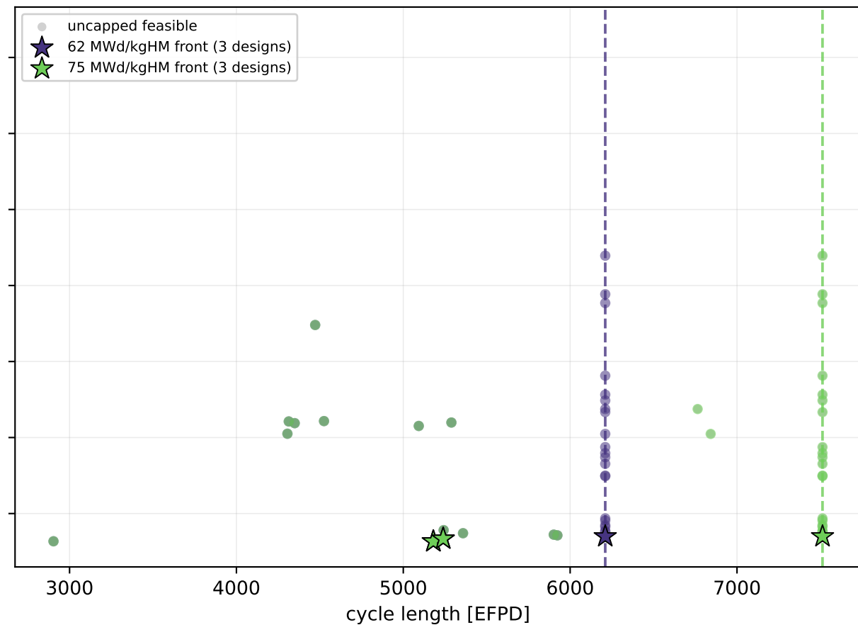
After applying the ATF discharge burnup limit
