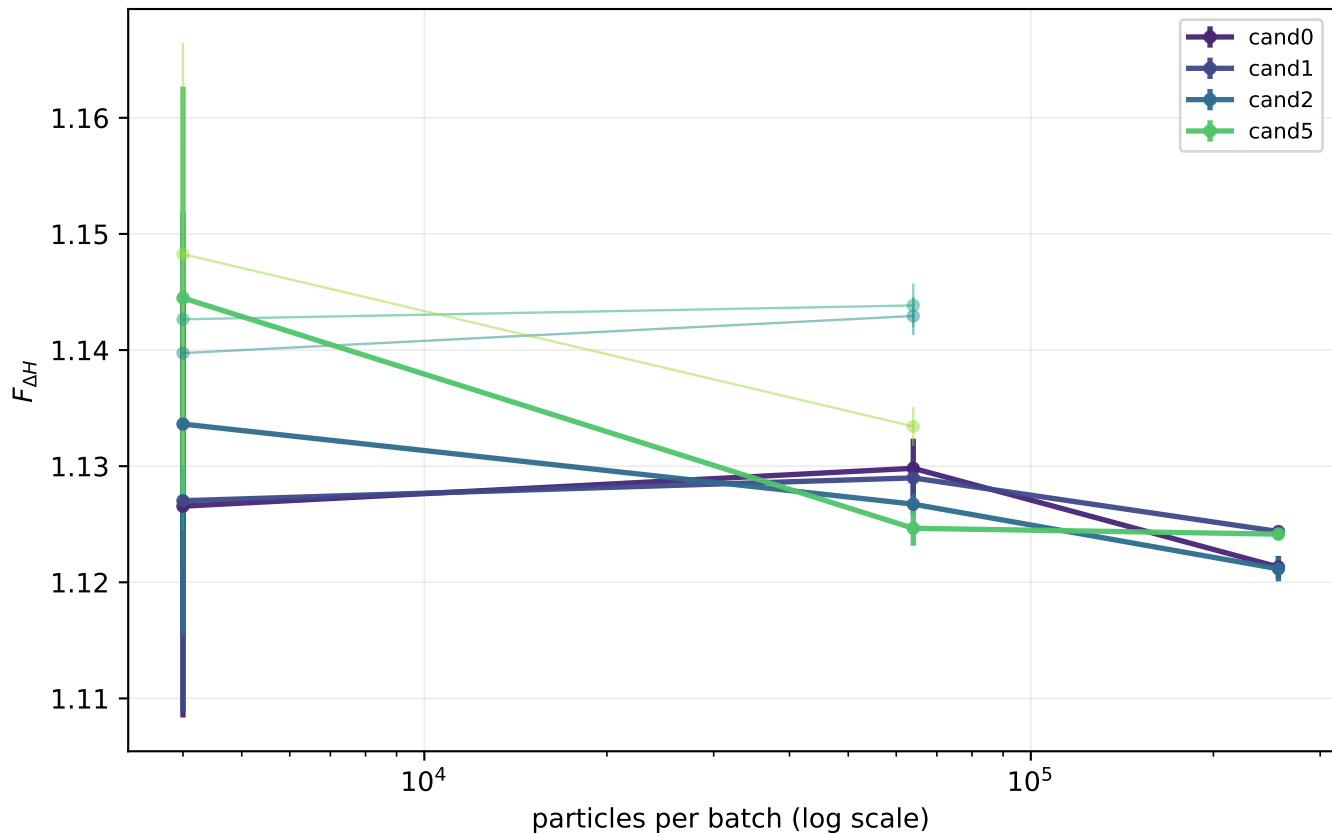
Max-over-cells estimator converges downward with fidelity (bias -0.0048 from 64000 to 256000 particles)
