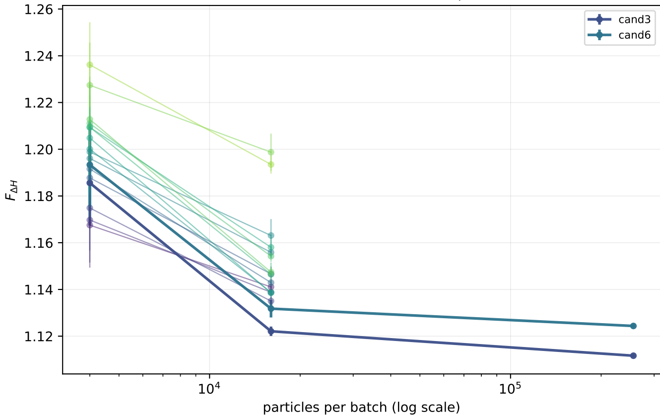
Max-over-cells estimator converges downward with fidelity (bias -0.0089 from 16000 to 256000 particles)
