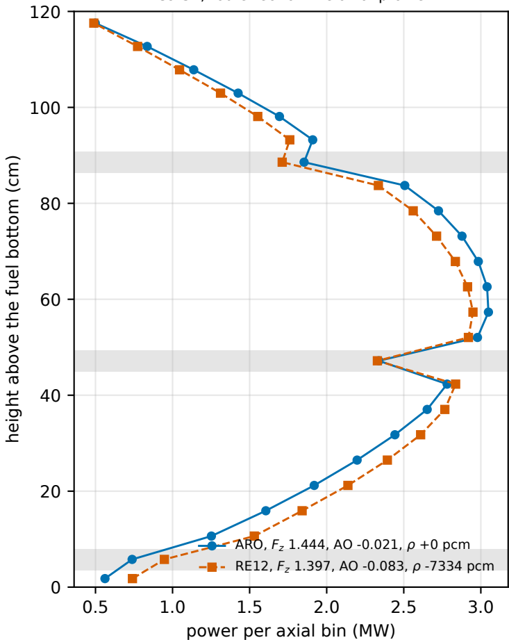
C9-34, rod effect on the axial profile
