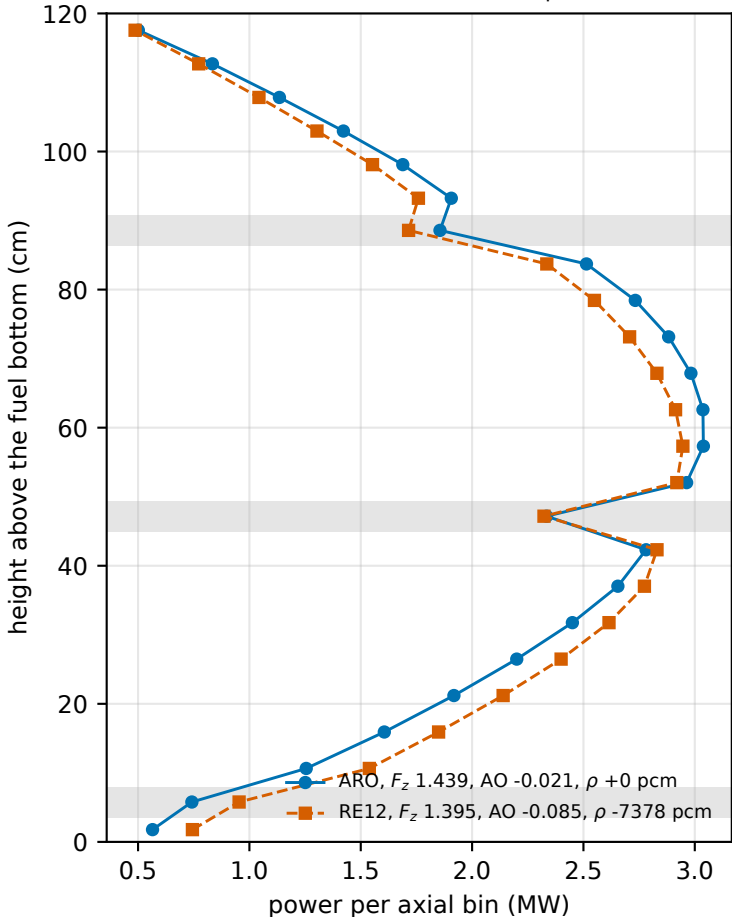
C9-44, rod effect on the axial profile
