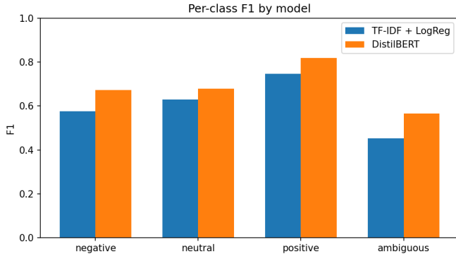
Figure 3: Per-class F1-scores on the test set.
