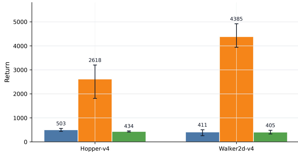
Final Return
