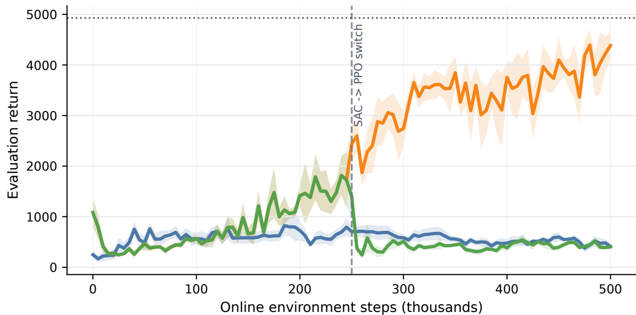
Walker2d-v4
