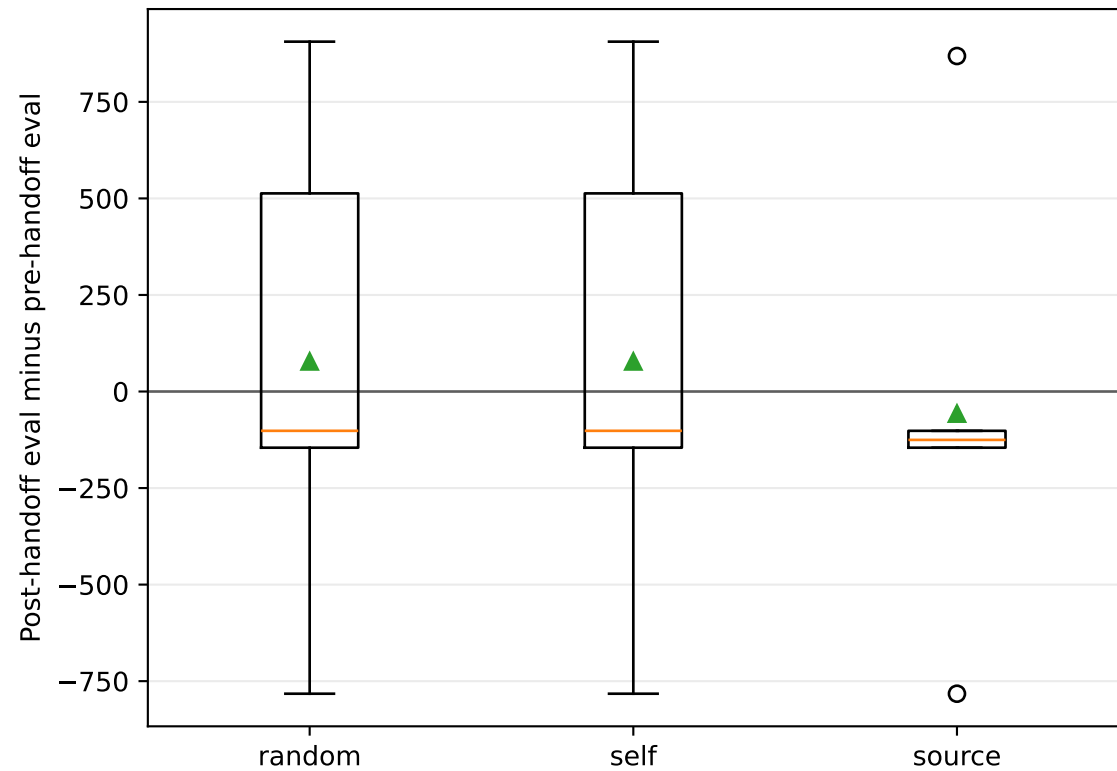
Walker2d-v4
