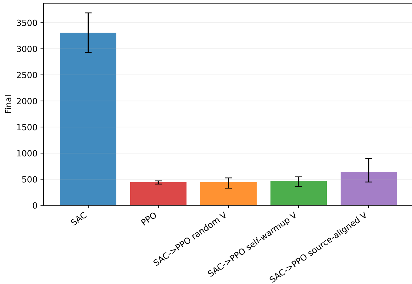
Walker2d-v4
