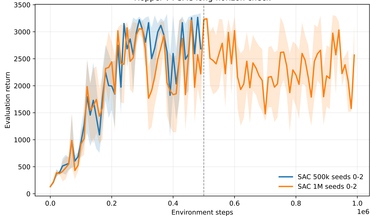
Hopper-v4 SAC long-horizon check
