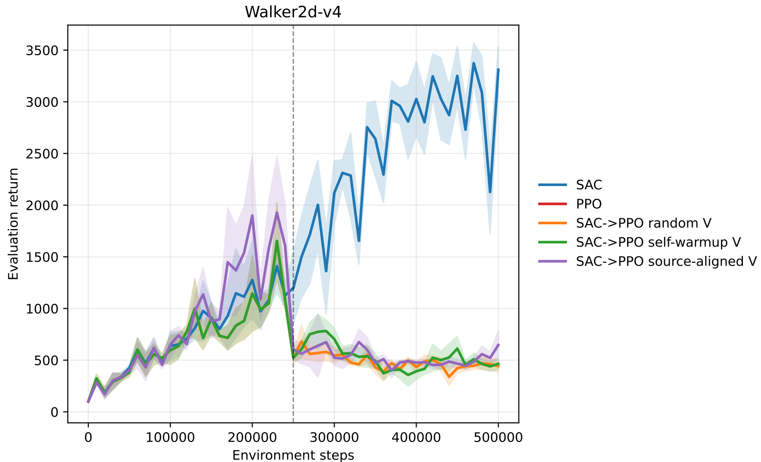
500k runs: mean evaluation return with standard error
