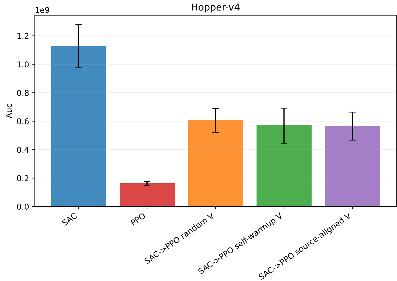
500k AUC by environment
