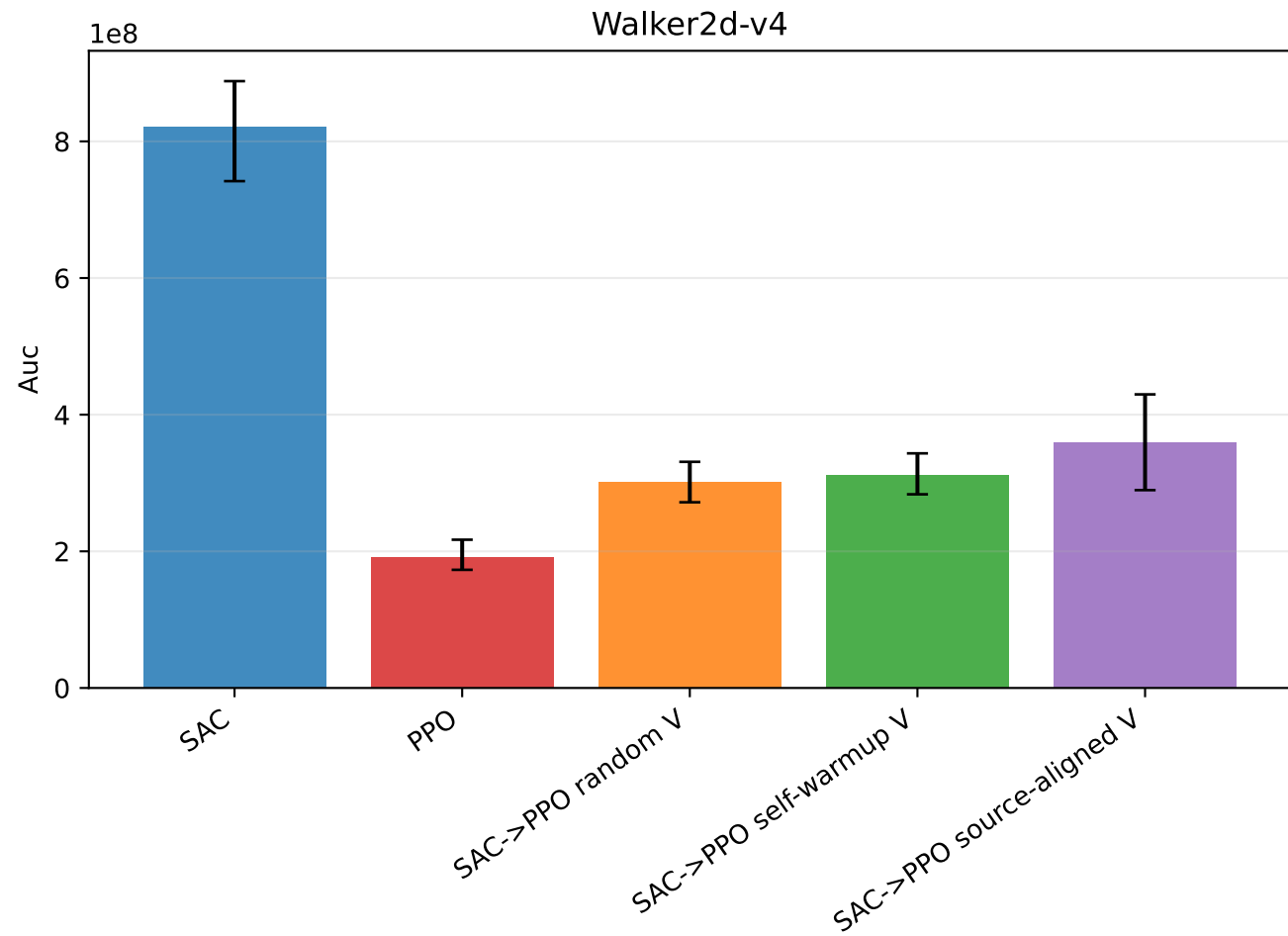
500k AUC by environment
