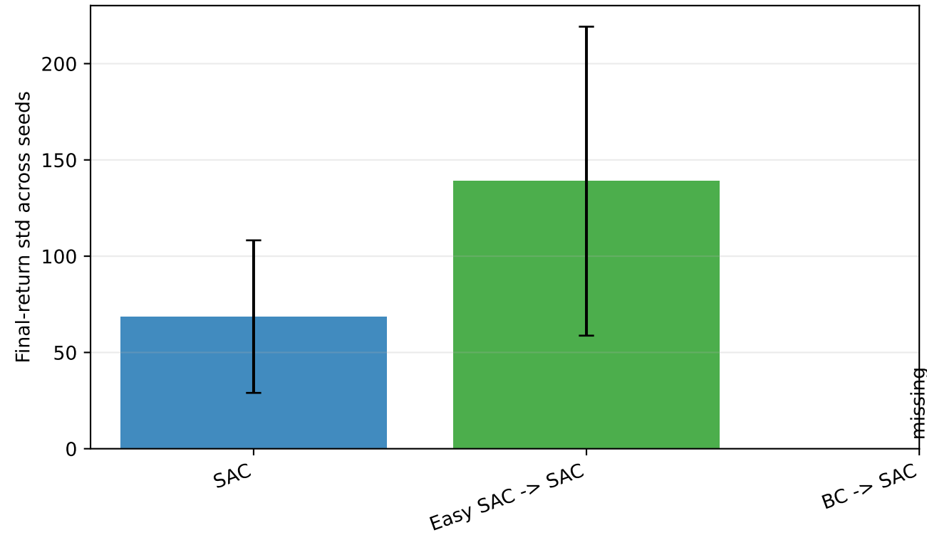
HalfCheetah-v4
