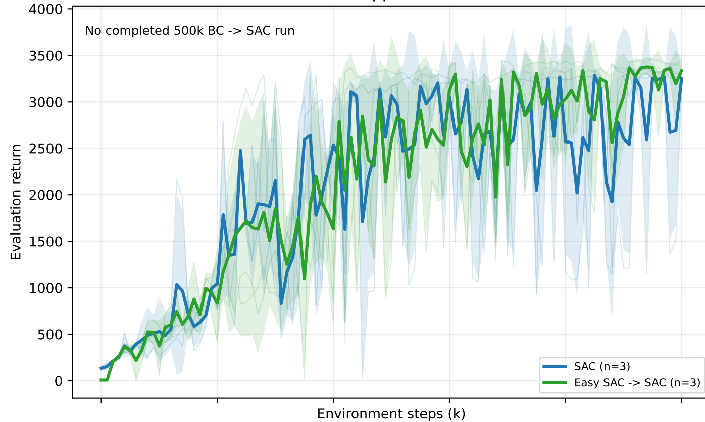
HalfCheetah-v4
