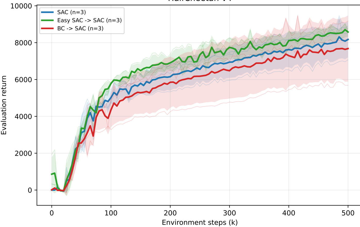
HalfCheetah-v4
