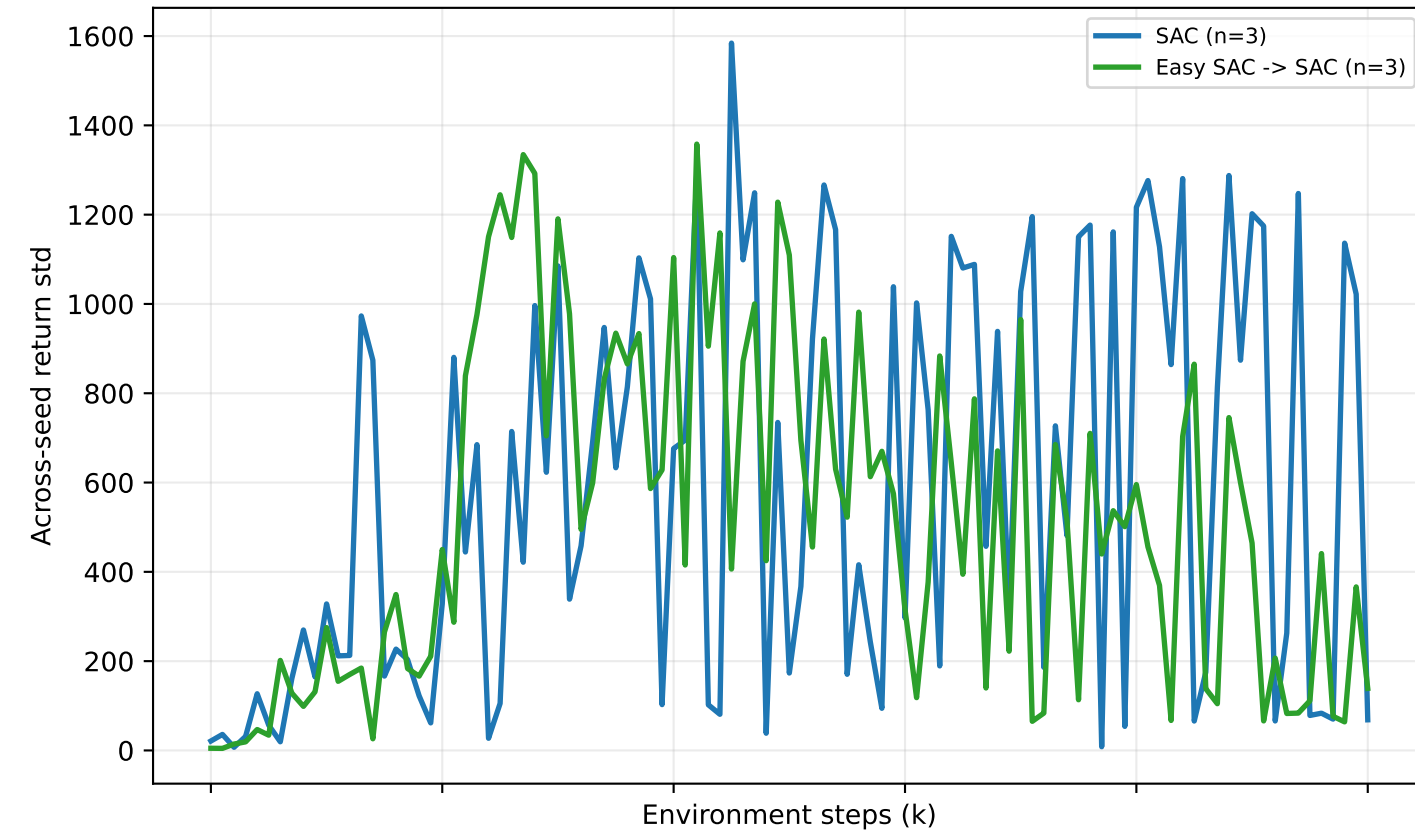
HalfCheetah-v4
