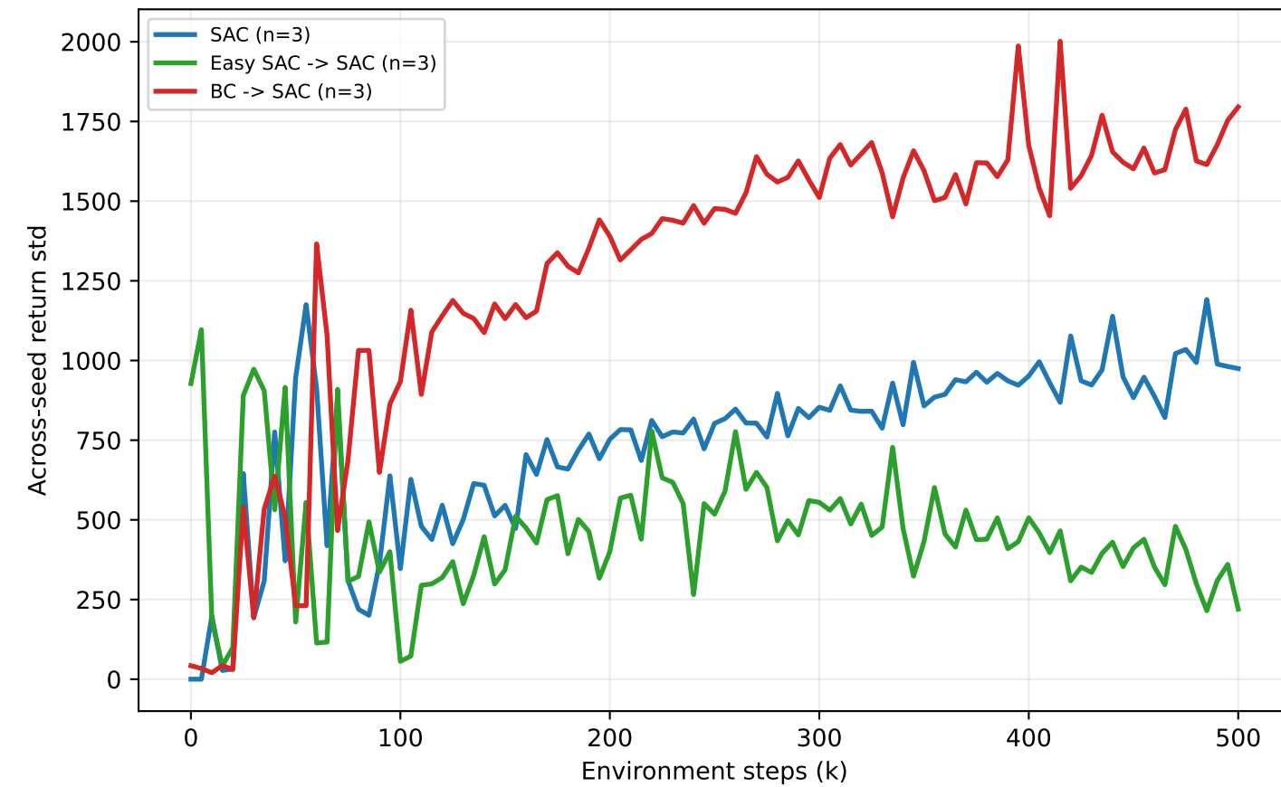
HalfCheetah-v4
