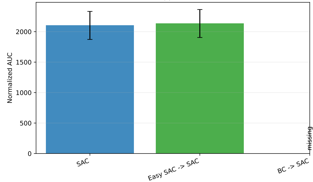
HalfCheetah-v4
