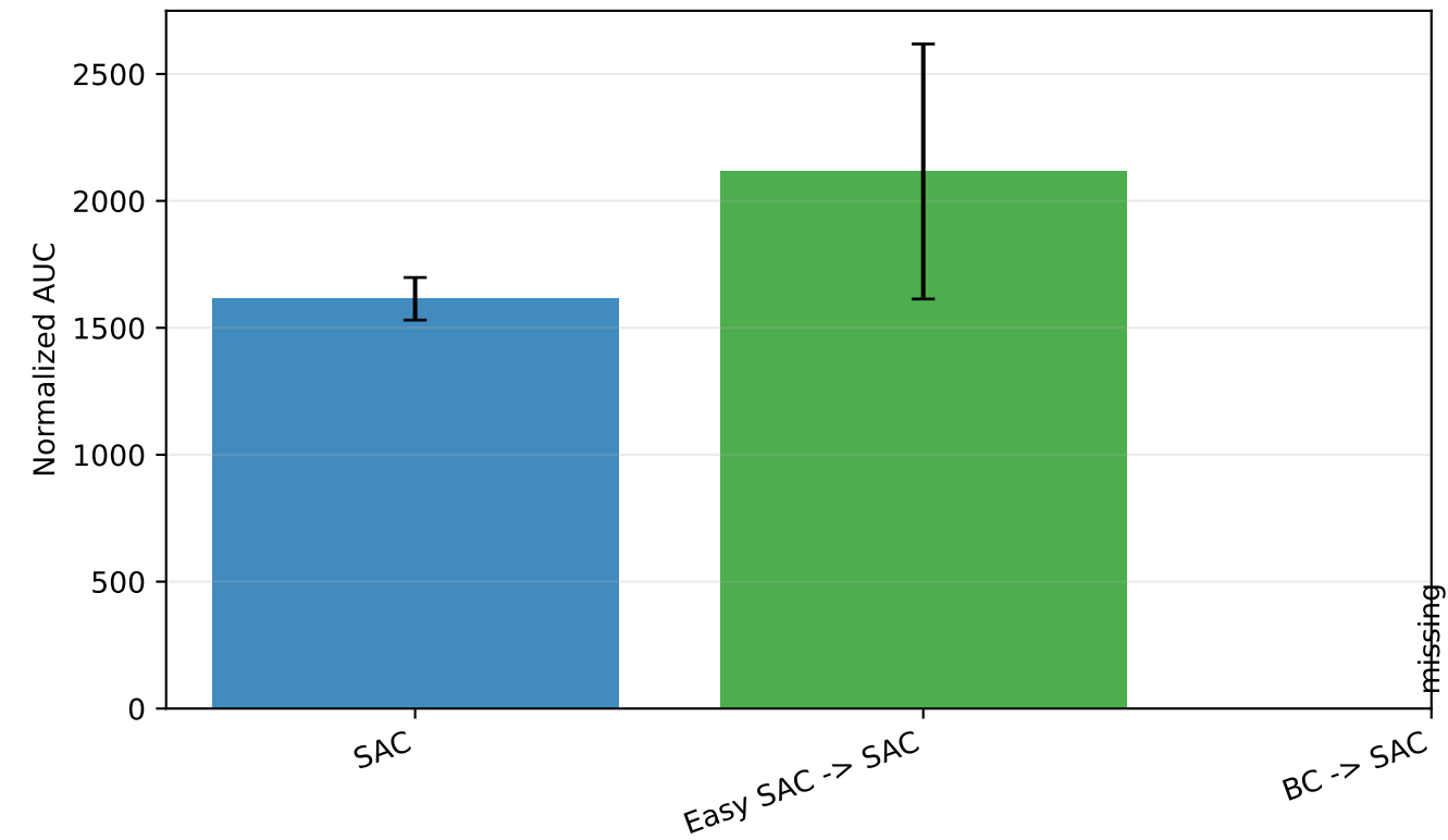
Walker2d-v4
