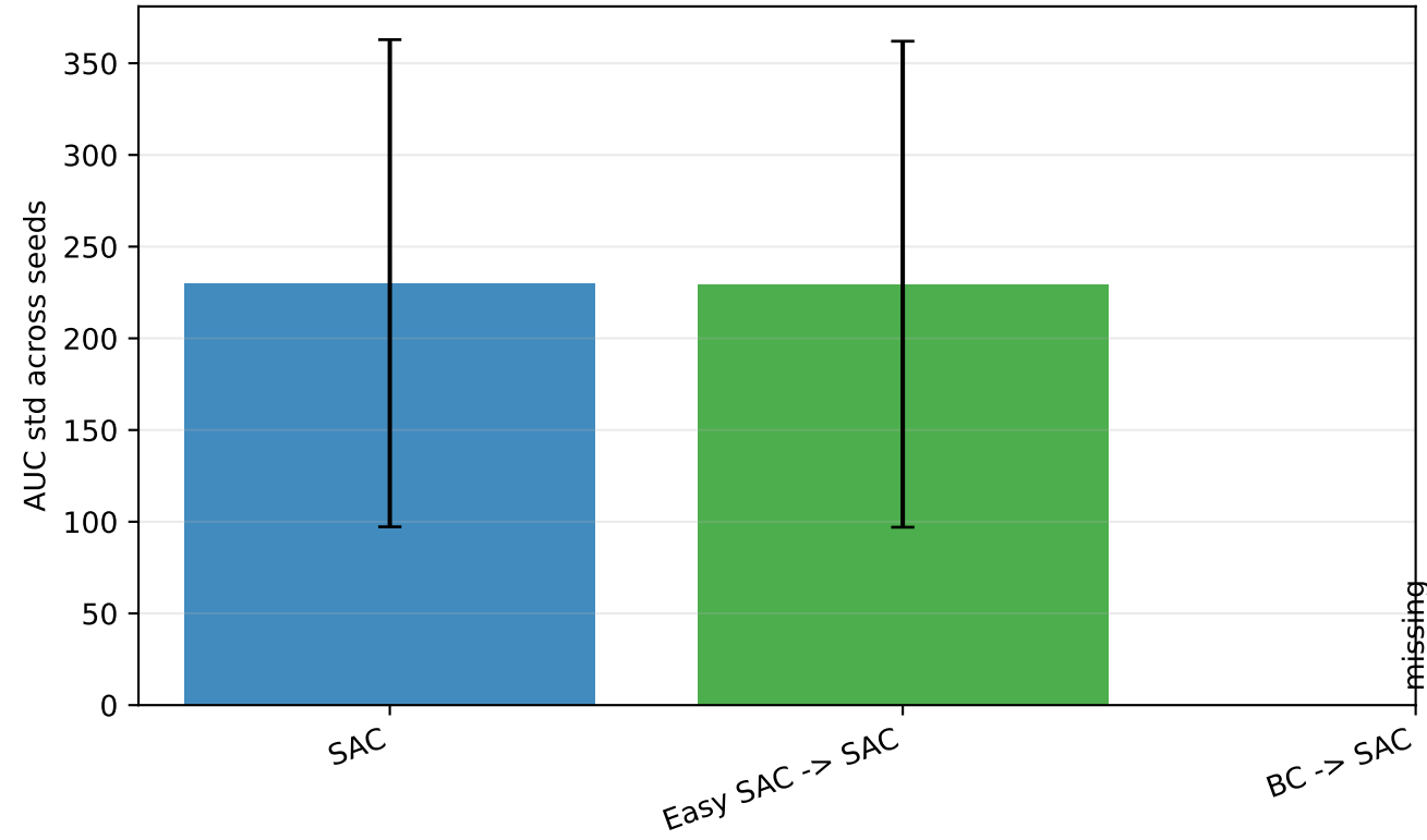
HalfCheetah-v4
