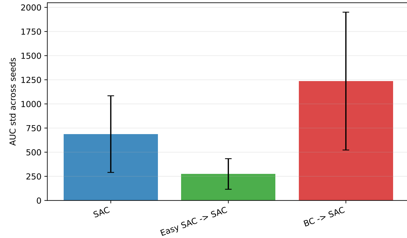
HalfCheetah-v4
