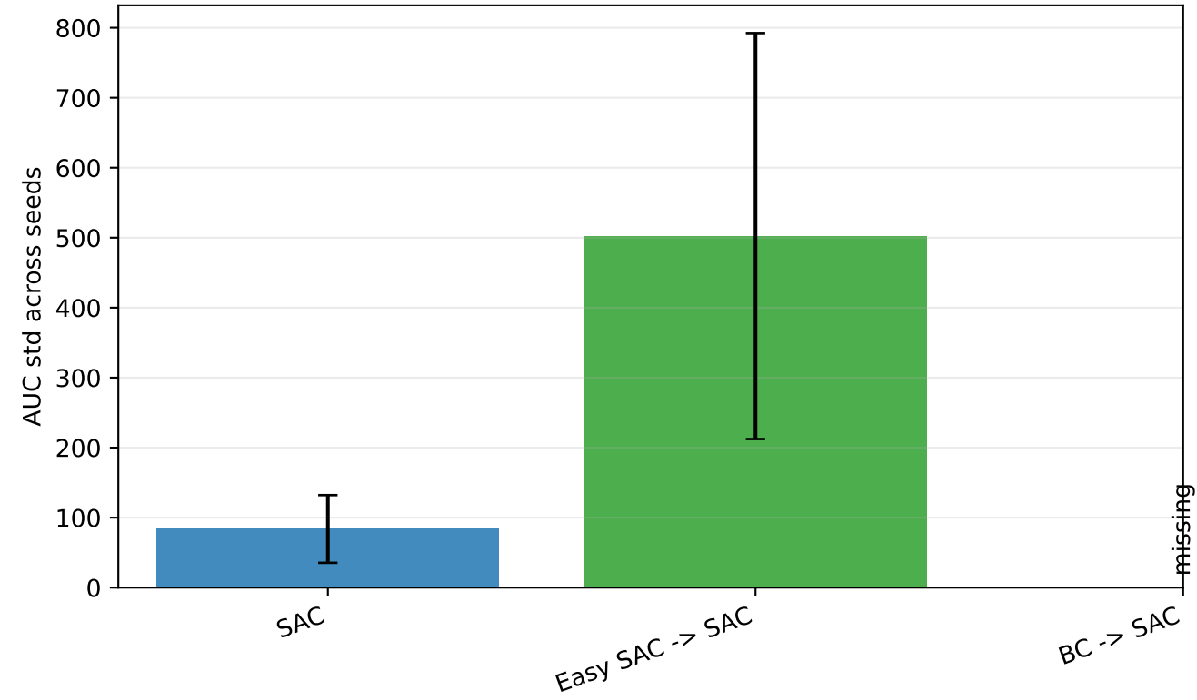
Walker2d-v4
