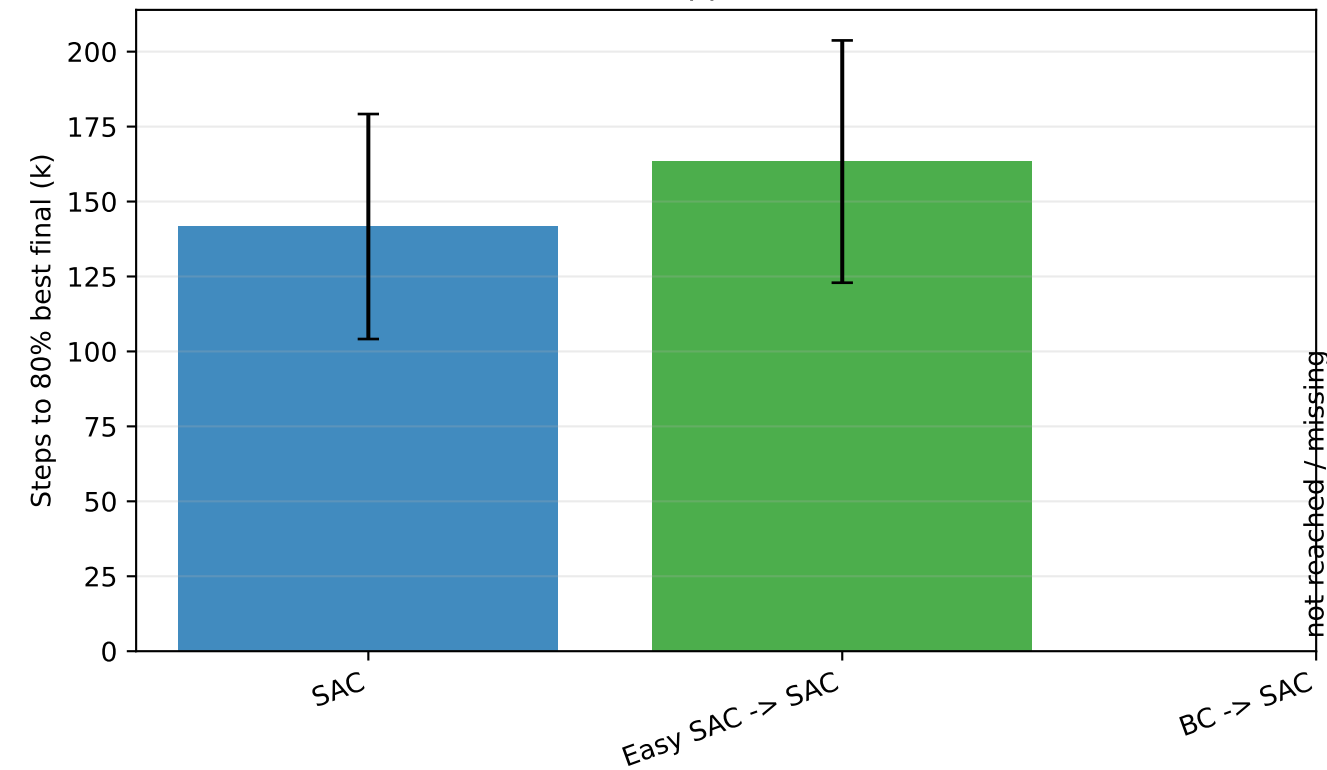
HalfCheetah-v4
