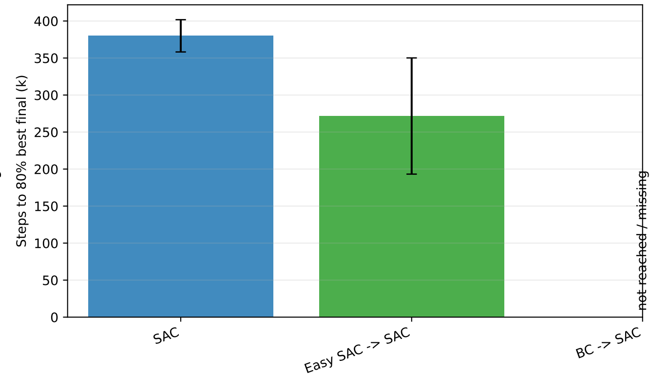
Walker2d-v4
