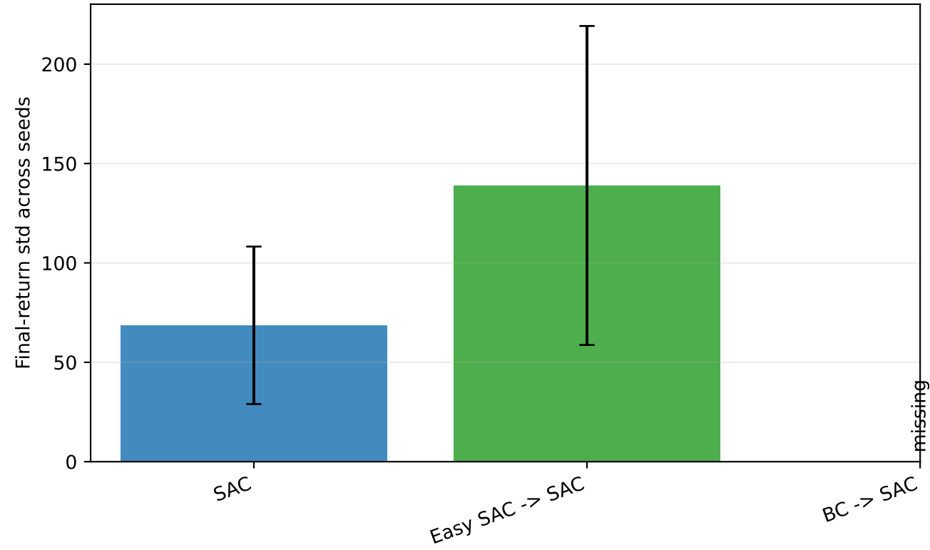
HalfCheetah-v4
