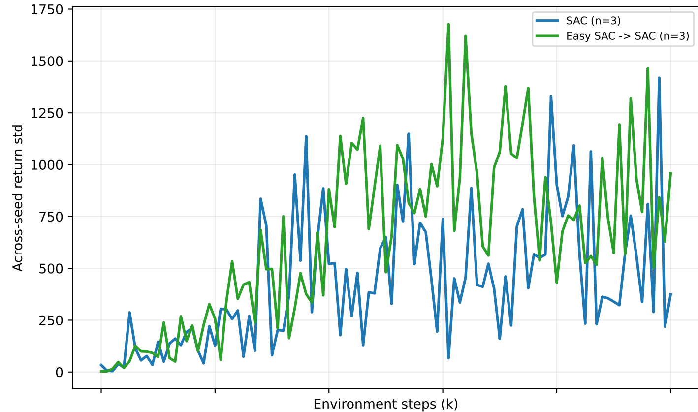
Walker2d-v4
