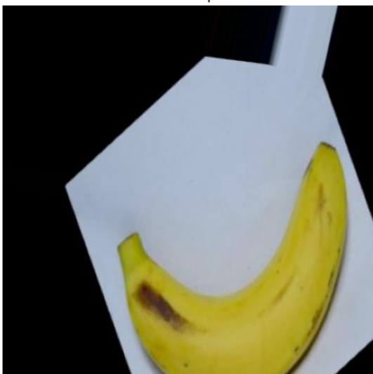
Class: ripe
