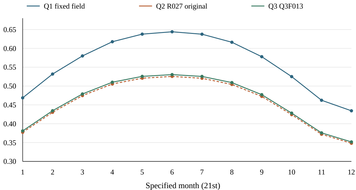
Sample mean thermal power per mirror area (kW/m 2 )
