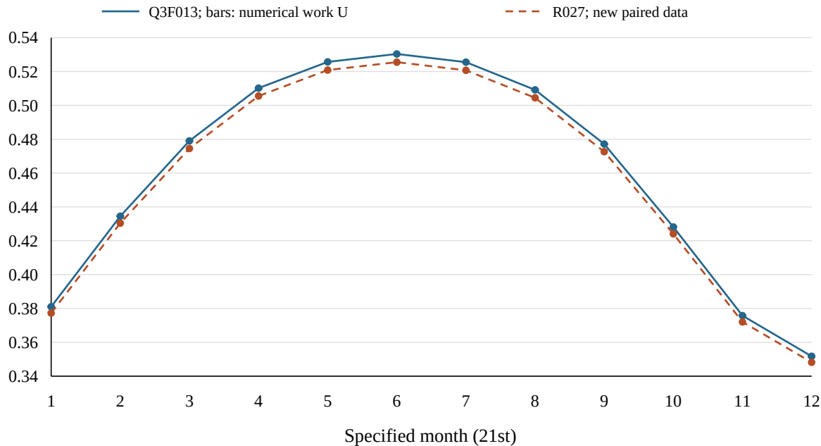
Sample mean thermal power per mirror area (kW/m 2 )
