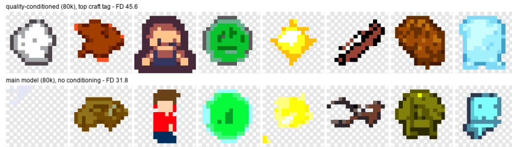
Figure 4: Quality conditioning at 16 px: same model, same prompts and seed, sampled with (top) and without (bottom) the top craft tag. The tagged samples are more finished and more detailed; both FD protocols rate them worse, because the tag narrows the distribution.
