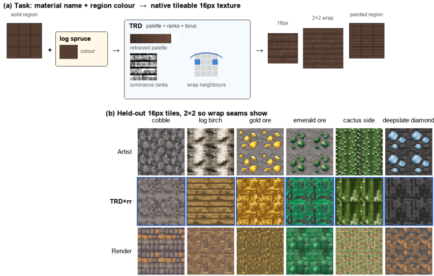
Figure 1: (a) The task. A material name and the region’s colour condition TRD, which decodes a retrieved palette and an N \times N luminance-rank grid under a toroidal relative bias and writes the tile into the region. (b) Held-out 16px name-to-texture samples ( 2 \times 2 so wrap seams are visible), chosen for variety from the materials on which the judge preferred TRD+rr over both Render and Retrieve. Unselected sheets are in Appendix E.
