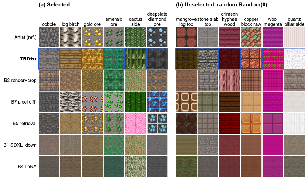
Figure 7: Name-only task; rows are methods, columns are test materials. (a) Selected: chosen by us for variety from the 70 of 272 test materials on which the judge preferred TRD+rr over both Render and Retrieve (both presentation orders agreeing). TRD keeps material-appropriate palettes and repeats seamlessly, whereas Shrink and LoRA wash out to near-uniform fills and Render’s crop can pick the wrong structure (cobble, cactus side). (b) Unselected: six of the 272 test materials drawn with a fixed seed ( random.Random(0) ) before looking at the samples, shown so that panel (a) can be read against typical outputs.
