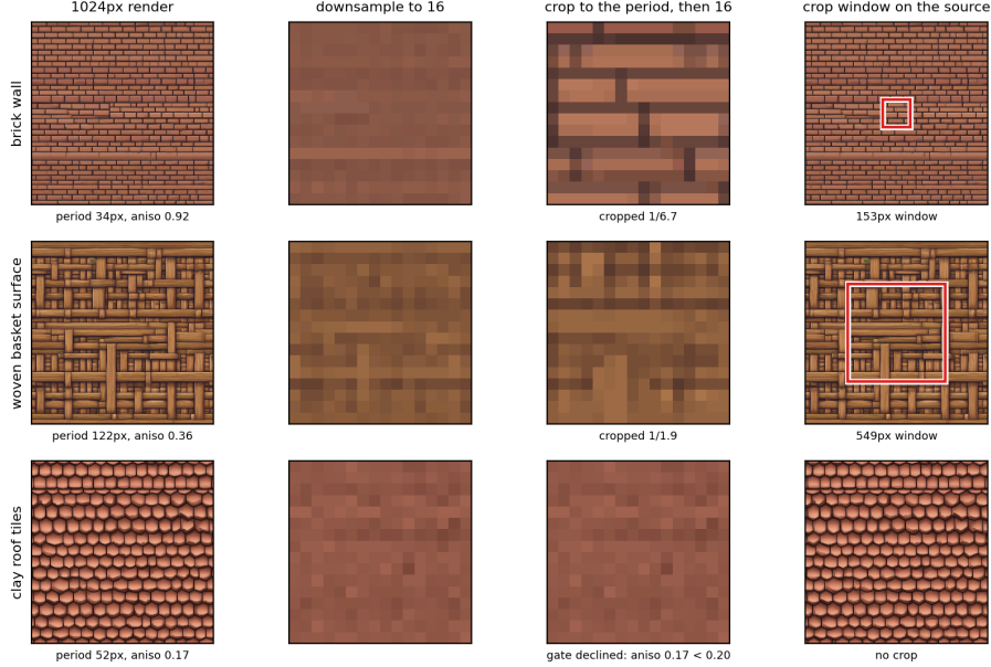
Figure 3: The strongest render-and-downsample baseline (Render). A 1024px render contains far more structural units than a 16px tile can hold, so plain downsampling (second column) loses the structure. Cropping to the detected period first (third column) repairs it when a period exists; an anisotropy gate declines to crop isotropic materials (bottom row). Because the crop is a fixed multiple of the period, the same window yields more detail at a larger target size, which is the canvas gain of §5.
