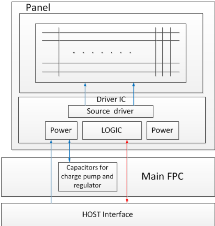
5.2.2 Display Module Block Diagram
