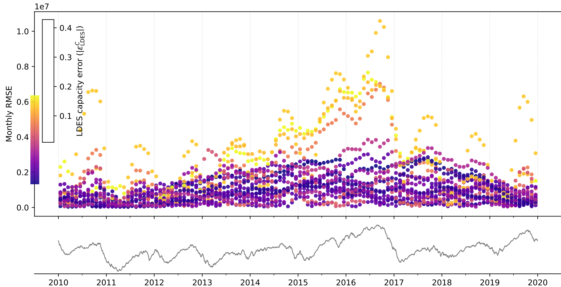
Monthly RMSE vs Reference SoC Proxy (colour = LDES capacity error)
