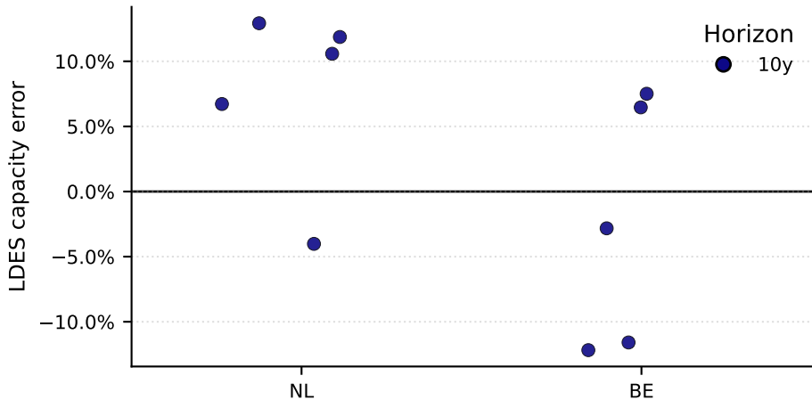
LDES capacity error | W=0.5 , reps=45, horizon=10y
