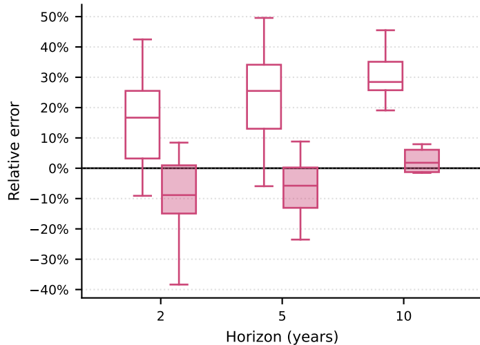
LDES capacity error
